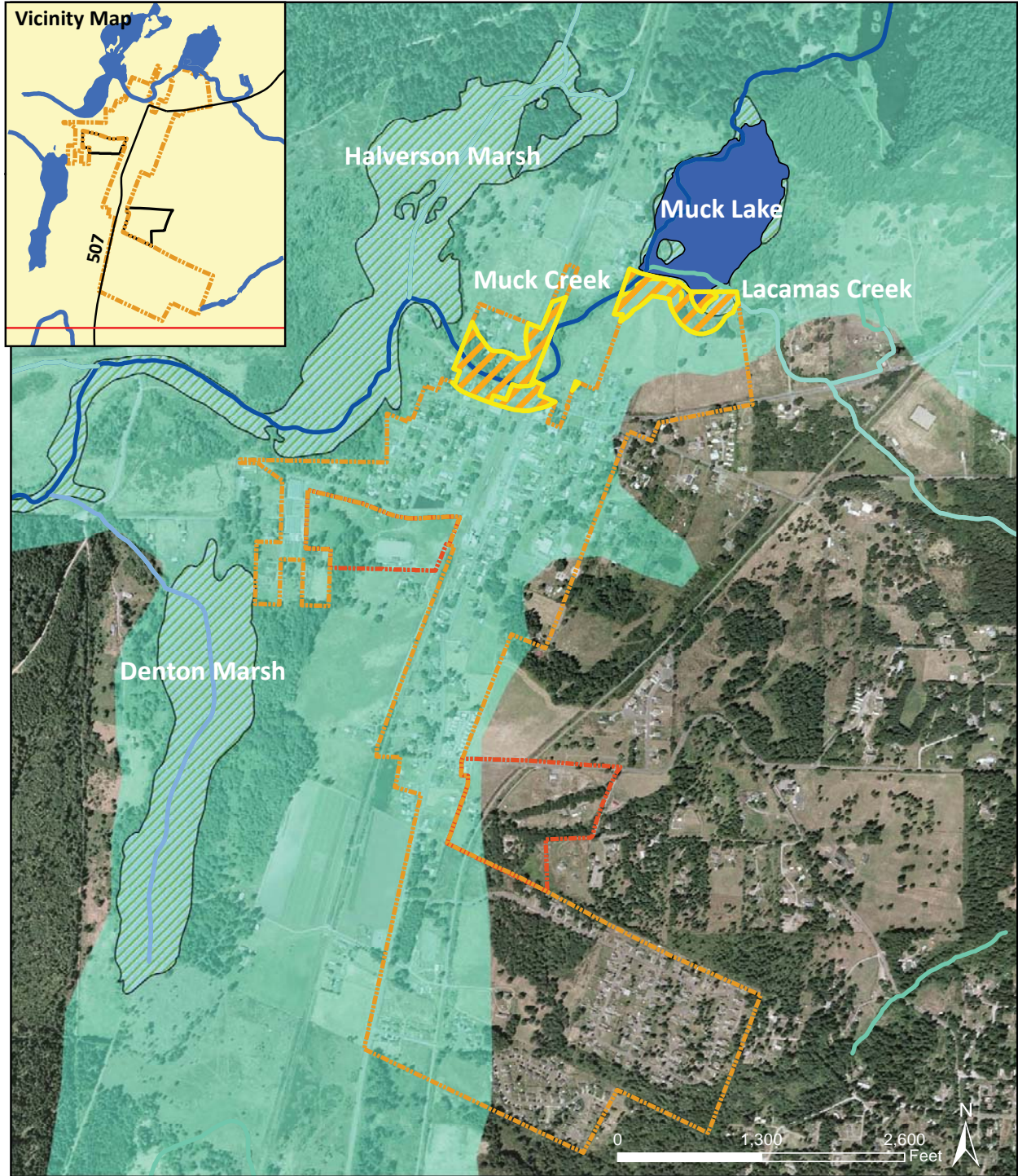
Figure 7 Aquifer Recharge Area
