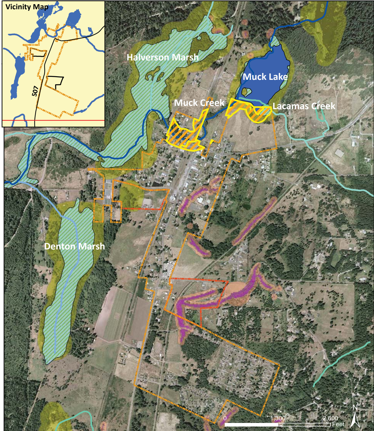
Figure 8 Steep Slopes, Potential Erosion & Landslide Hazard Areas
