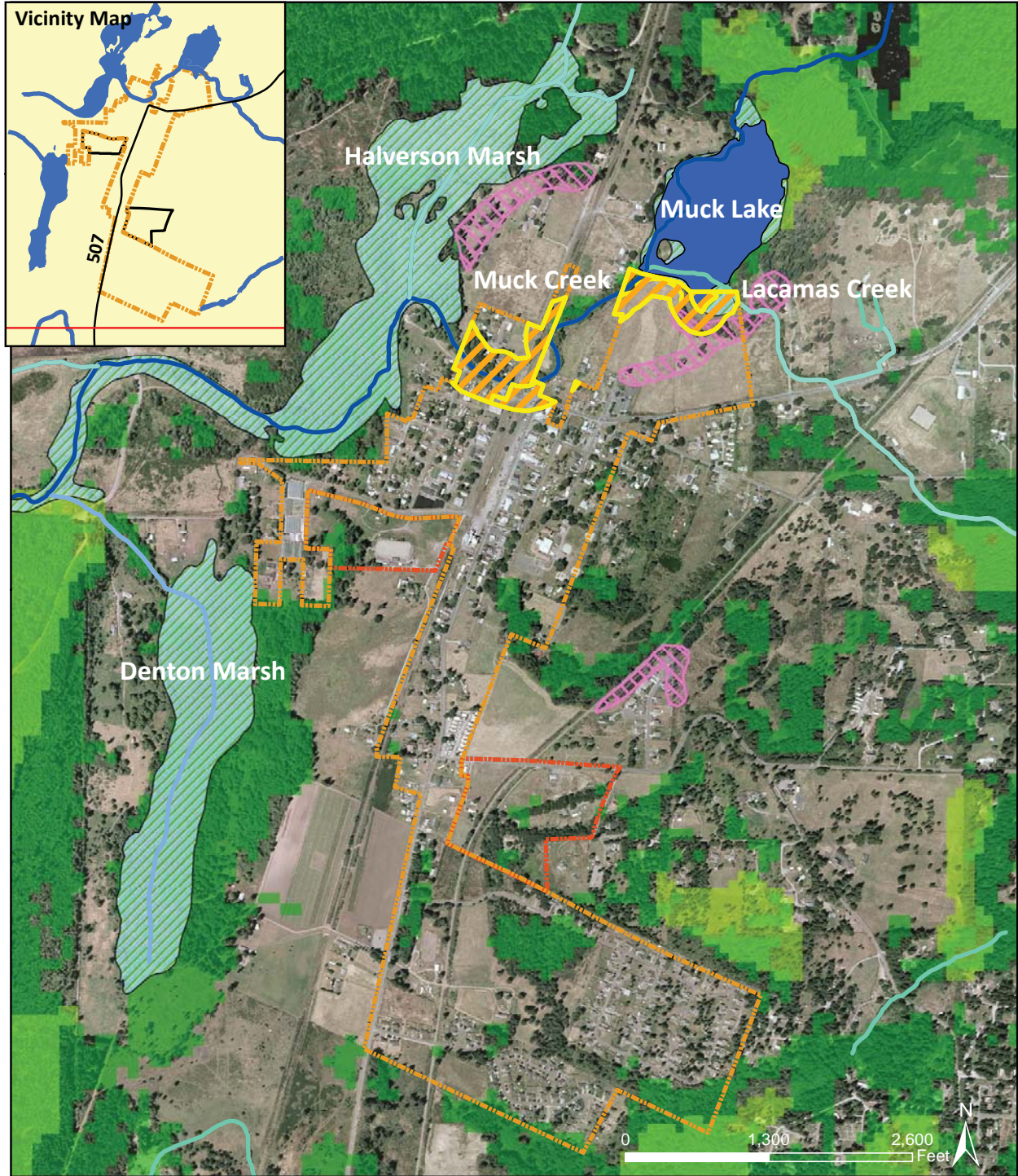
Figure 10 Forest and Canopy Coverage
